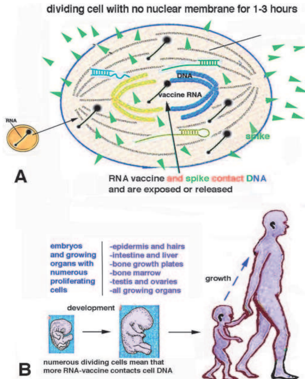
Fig. 4. Contact of vaccine RNA with chromosomes (DNA) during mitosis (A), and unknown consequences on bodies containing many dividing cells that can incorporate high amount of biotech-RNA (B). A, dividing cell containing both biotech-RNAs and their coded spike proteins that are distributed in the cytoplasm and nuclear region contacting the chromosomes (DNA). Spike proteins or their fragments (peptides) are exposed on the cell surface or released extracellularly. B, embryos, fetuses, growing children and young individuals contain many dividing cells so that the uptake of biotech-RNA or-DNA is higher than in fully grown-up adult or elderly individuals where a lower number of dividing cells are present. Main affected tissues are physiologically renewal tissues, and some are indicated.
