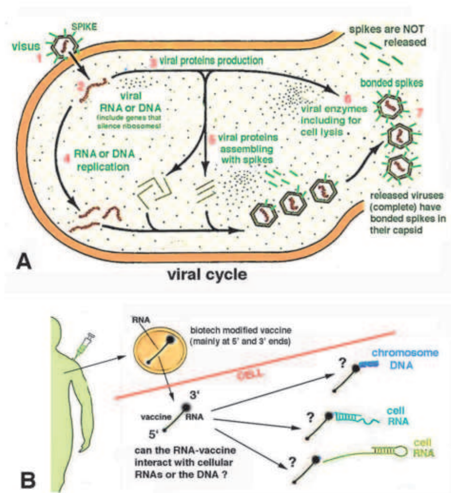
Fig. 3. Classic viral cycle (A) and biotech-RNA vaccine potential interactions within cells. A , after viral infection, new viral particles are release complete, with spikes attached to the capsid, not released as soluble spike proteins. B , after RNA-vaccine (black bar with main modification in the 5' and 3' nucleotide ends of the RNA) injection and penetration into various cells, potential interaction (?) with cellular RNAs or DNA remain unknown because of incomplete knowledge of all cellular functions.
